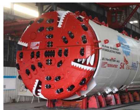
PHOTO >> TERRATEC HARD ROCK TBM
